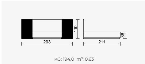
Toronto Bedstead (160) WITH DRAWERS
